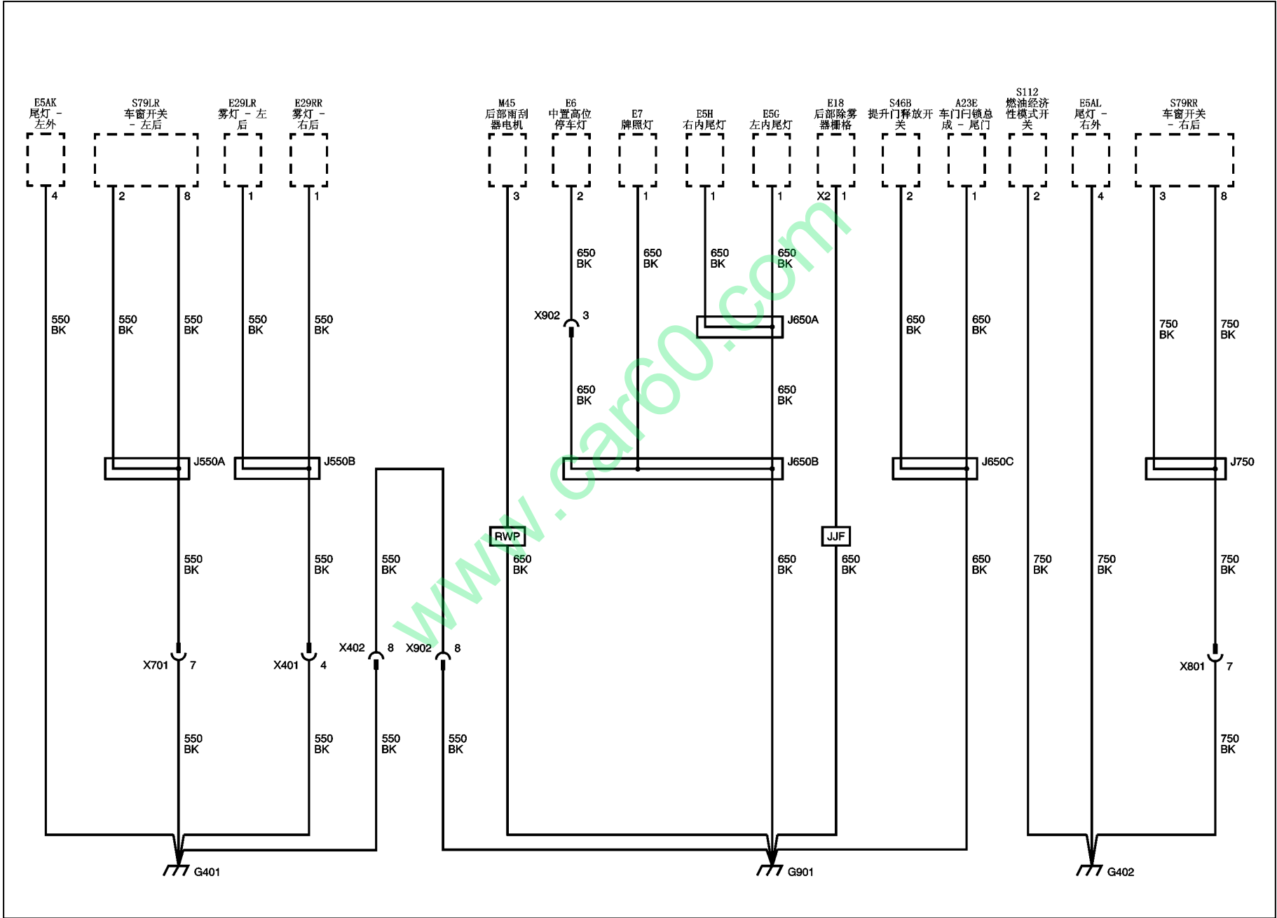
搭铁示意图 (G401, G402, G901 搭铁)
