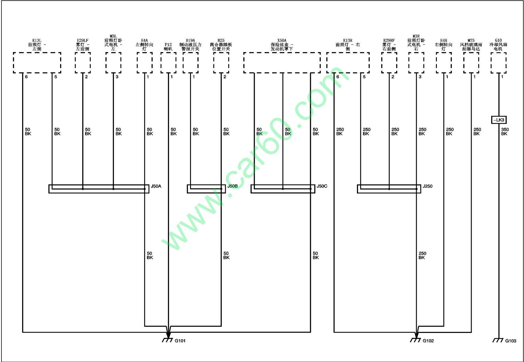
搭铁示意图 (G101, G102, G103 搭铁)
